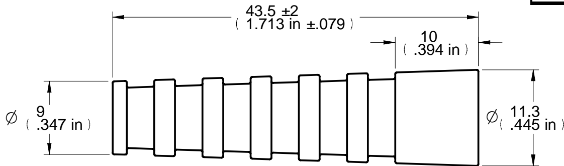
DIM OUTLINE
