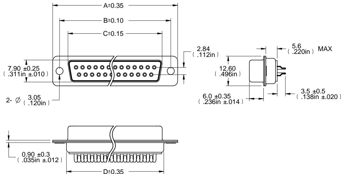
DIM OUTLINE
